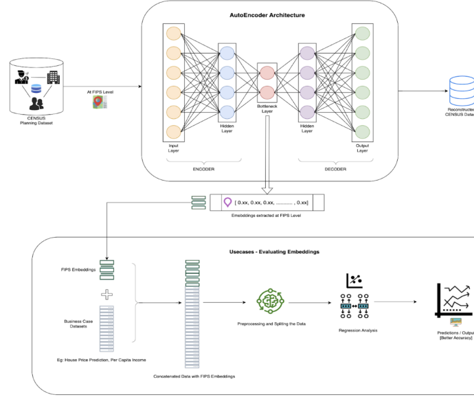
Fig. 1. Architecture of the Autoencoder model utilized for dimensionality reduction in census data analysis, showing the flow from input to compressed representation at the bottleneck layer, and reconstruction at the output.
