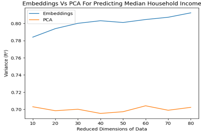
Fig. 3. Comparison of R-squared scores for PCA and Autoencoder embeddings across different dimensions
